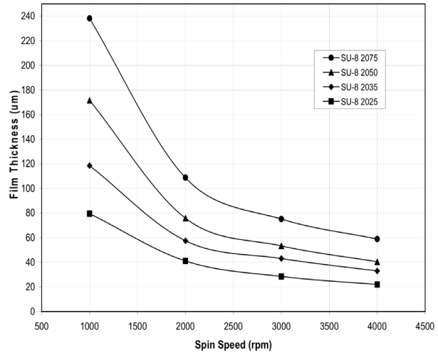
Figure 1. SU-8 2000 Spin Speed vs. Thickness
