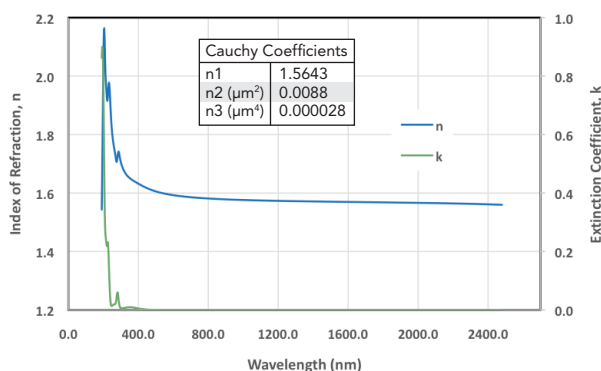
Figure 2. Cauchy Coefficients
