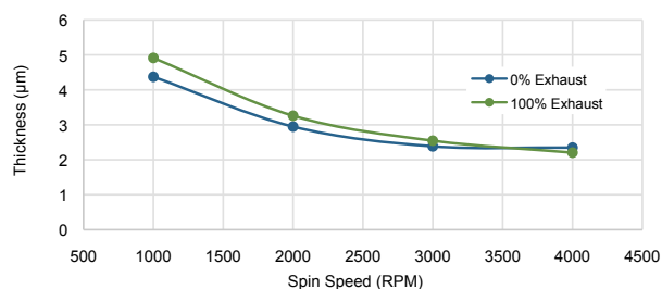
Figure 1C. UniLOR™ N 3.5 Spin Speed Curve
