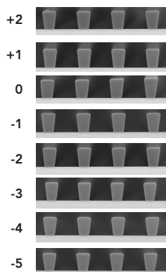
Figure 6. Depth of Focus Study
