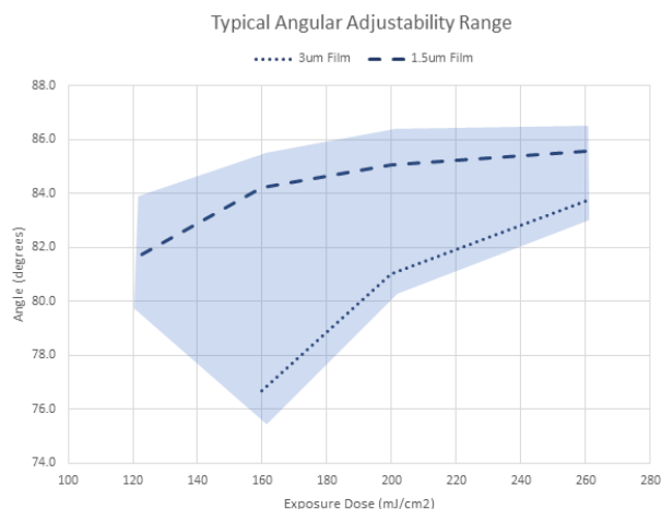
Figure 4. Process Window of Variable Exposure Doses in 1.5 \mu\text{m} and 3 \mu\text{m} Film Thicknesses on Si
