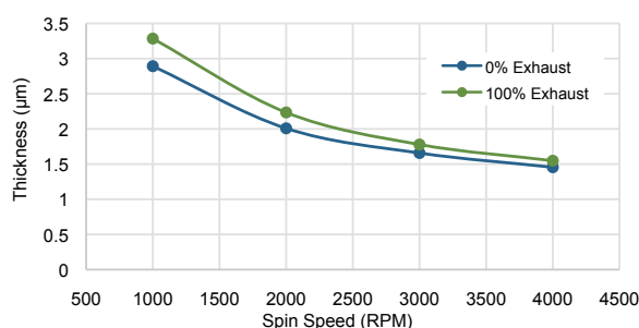
Figure 1B. UniLOR™ N 2.5 Spin Speed Curve
