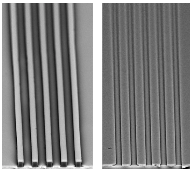
3 µm L/S before/after lift-off of 4000 Å evaporated Aluminum deposition on 2.5 µm thick film
