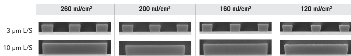
Figure 3: Varying Exposure Dose of 3 and 10 \mu\text{m} L/S in 1.5 \mu\text{m} Thick Film
