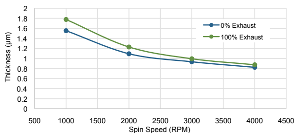
Figure 1A. UniLOR™ N 1.5 Spin Speed Curve
